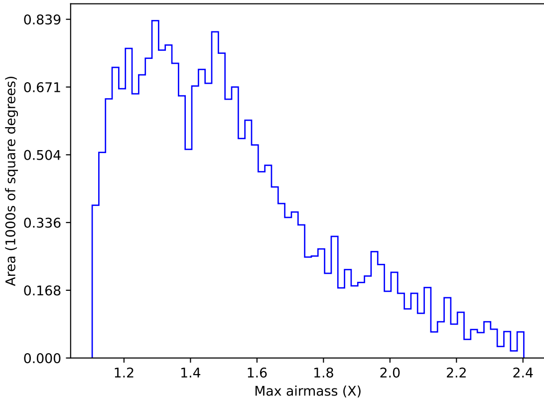
ddf_loaded_half_f18_v3.4_10yrs Yr 1 u band: Max airmass
