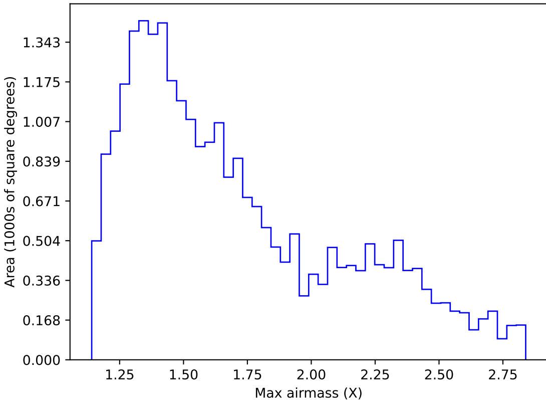
ddf_loaded_half_fl8_v3.4_10yrs Yr 1 i band: Max airmass
