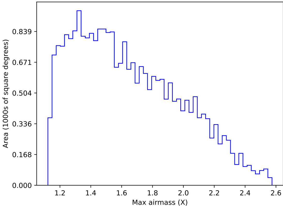
ddf_loaded_half_fl8_v3.4_10yrs Yr 1 g band: Max airmass
