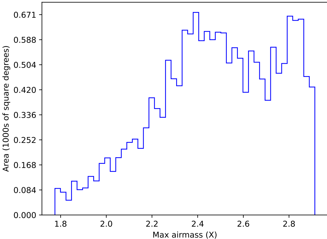
ddf_loaded_half_fl8_v3.4_10yrs WFD z band: Max airmass
