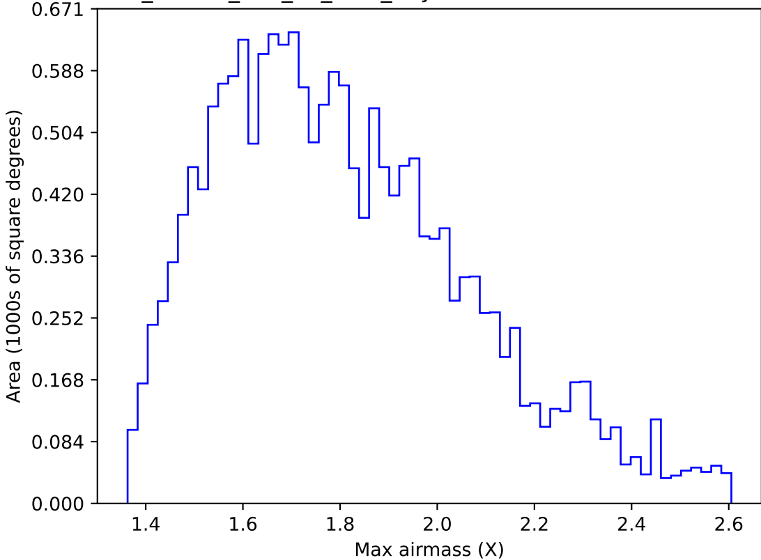
ddf_loaded_half_fl8_v3.4_10yrs WFD u band: Max airmass
