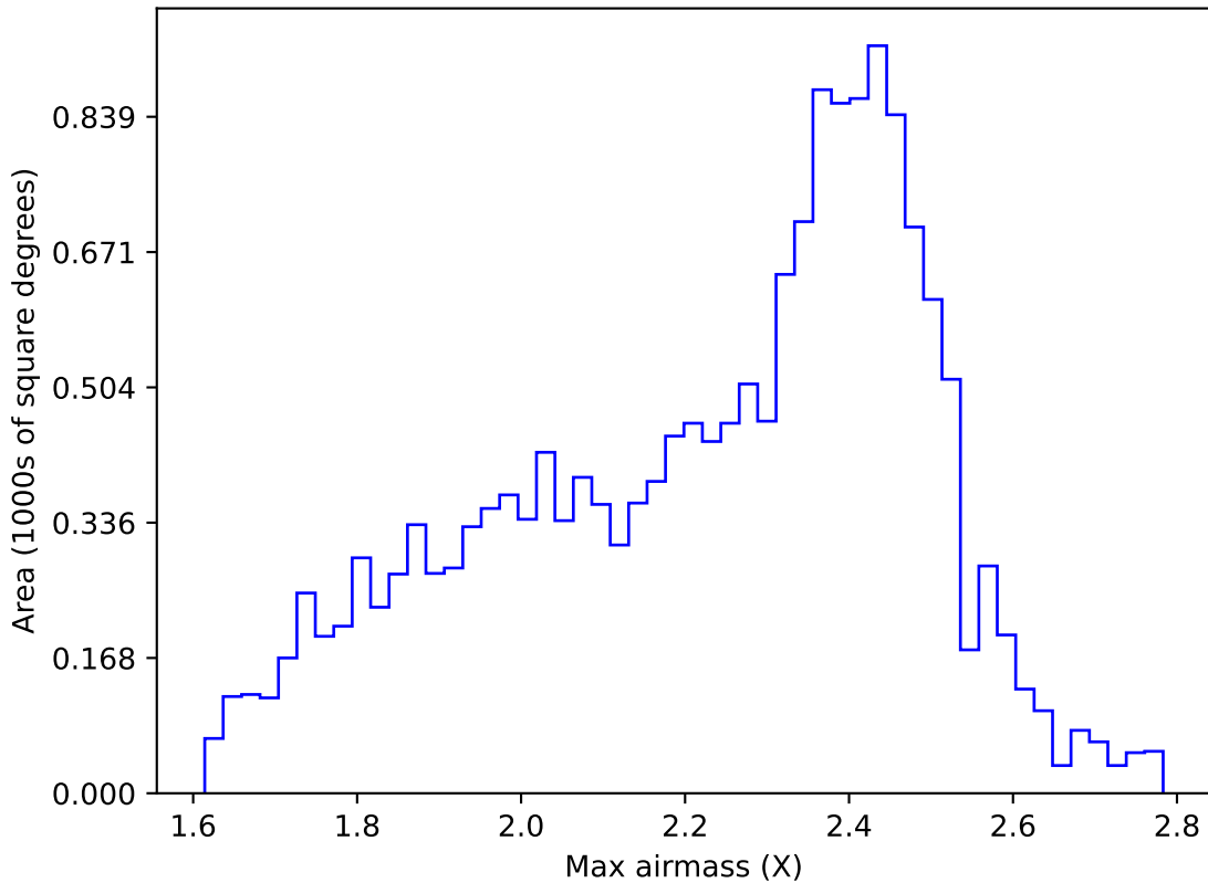
ddf_loaded_half_f18_v3.4_10yrs WFD r band: Max airmass
