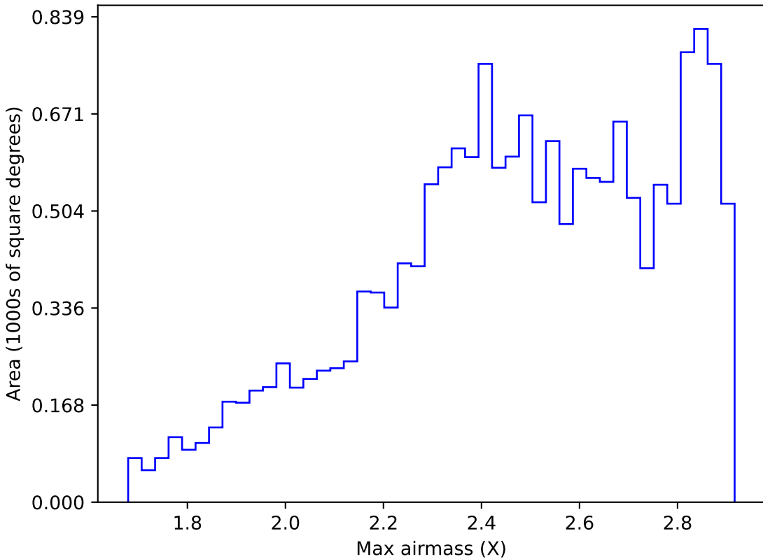
ddf_loaded_half_f18_v3.4_10yrs WFD i band: Max airmass
