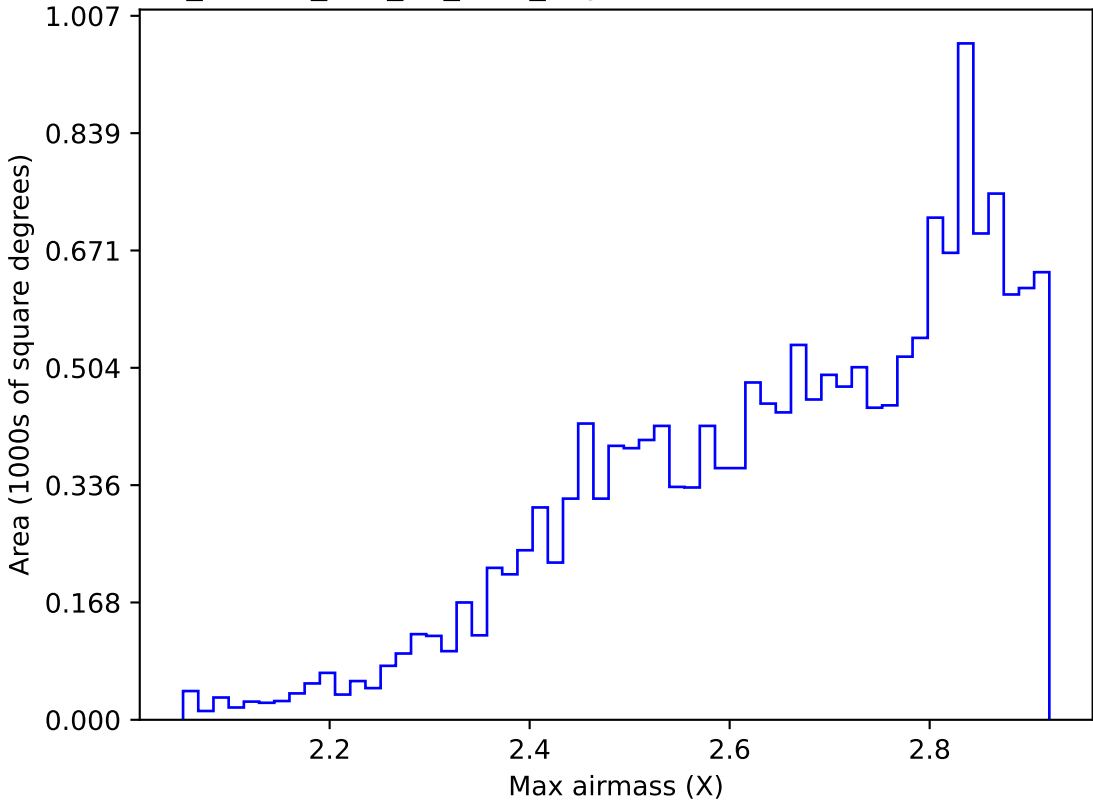
ddf_loaded_half_fl8_v3.4_10yrs WFD all bands: Max airmass
