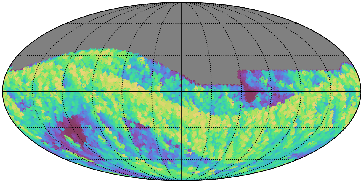
ddf_loaded_half_fl8_v3.4_10yrs All sky z band: Max airmass
