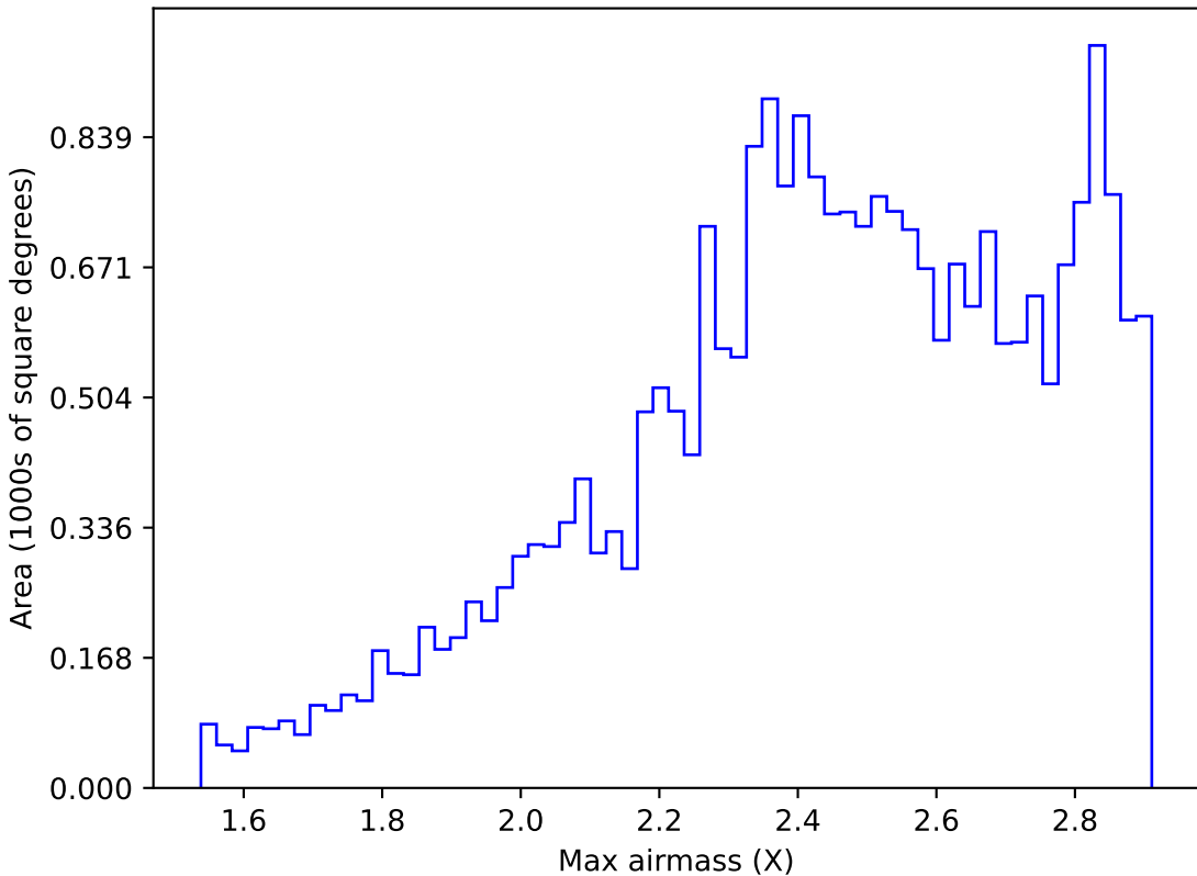
ddf_loaded_half_fl8_v3.4_10yrs All sky z band: Max airmass
