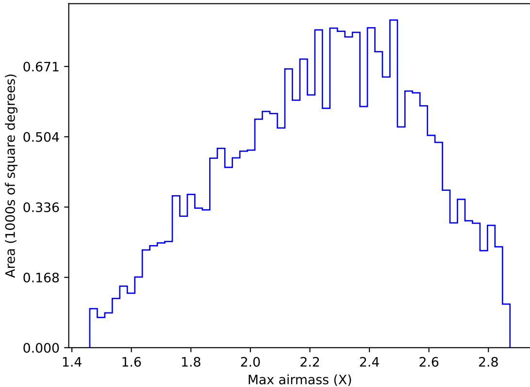
ddf_loaded_half_fl8_v3.4_10yrs All sky y band: Max airmass
