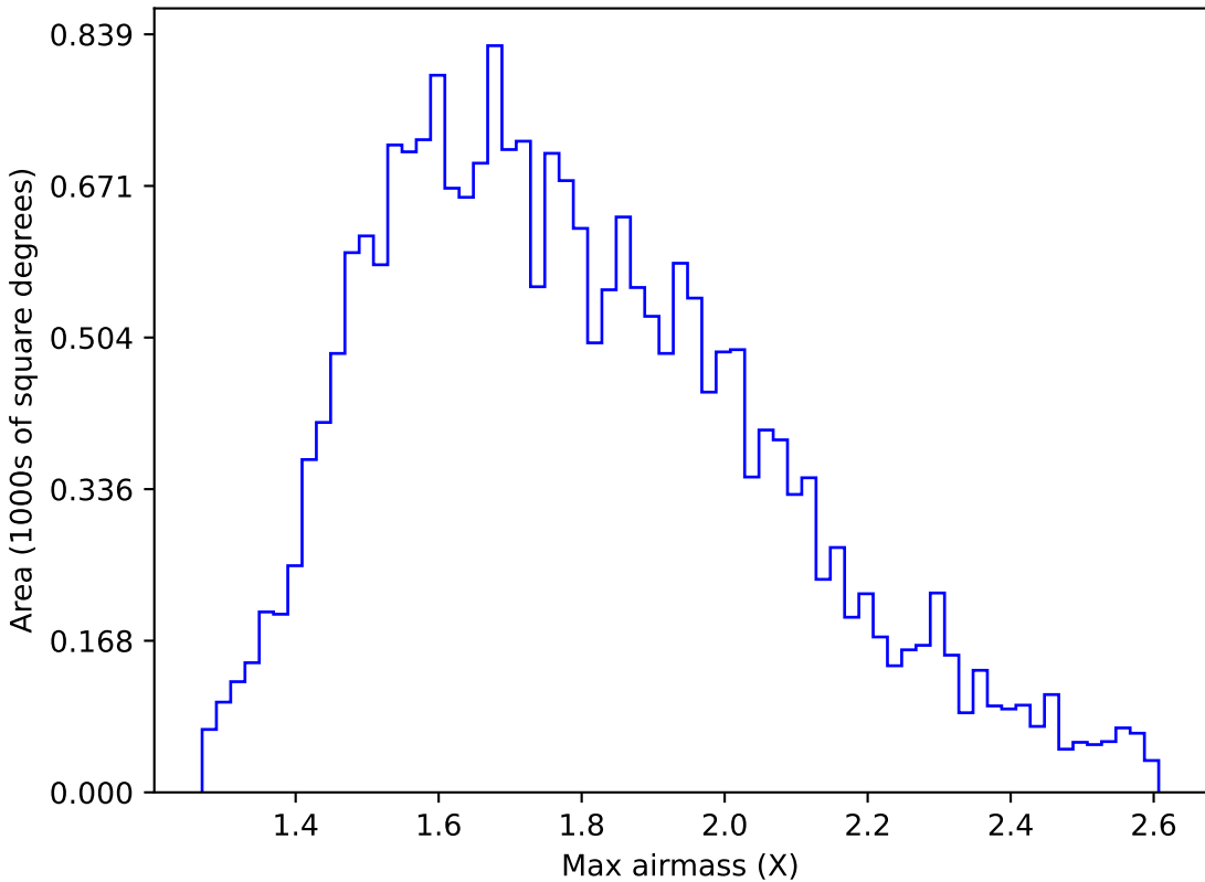
ddf_loaded_half_fl8_v3.4_10yrs All sky u band: Max airmass
