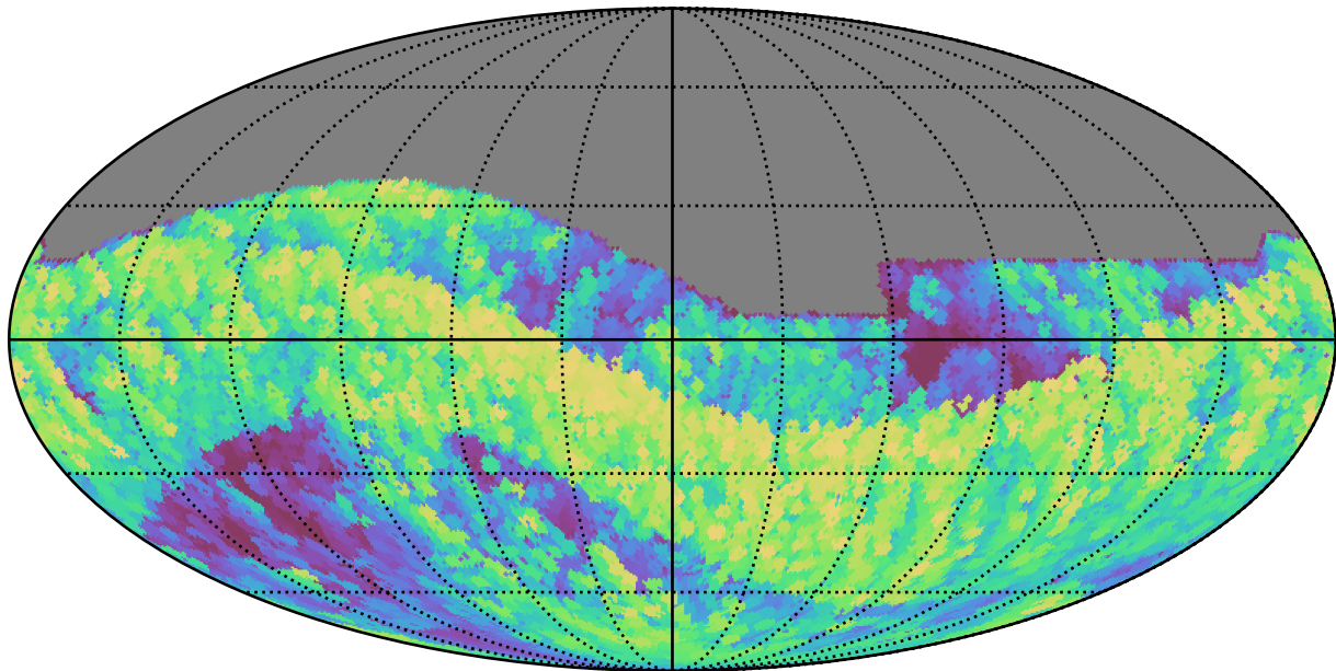
ddf_loaded_half_fl8_v3.4_10yrs All sky i band: Max airmass
