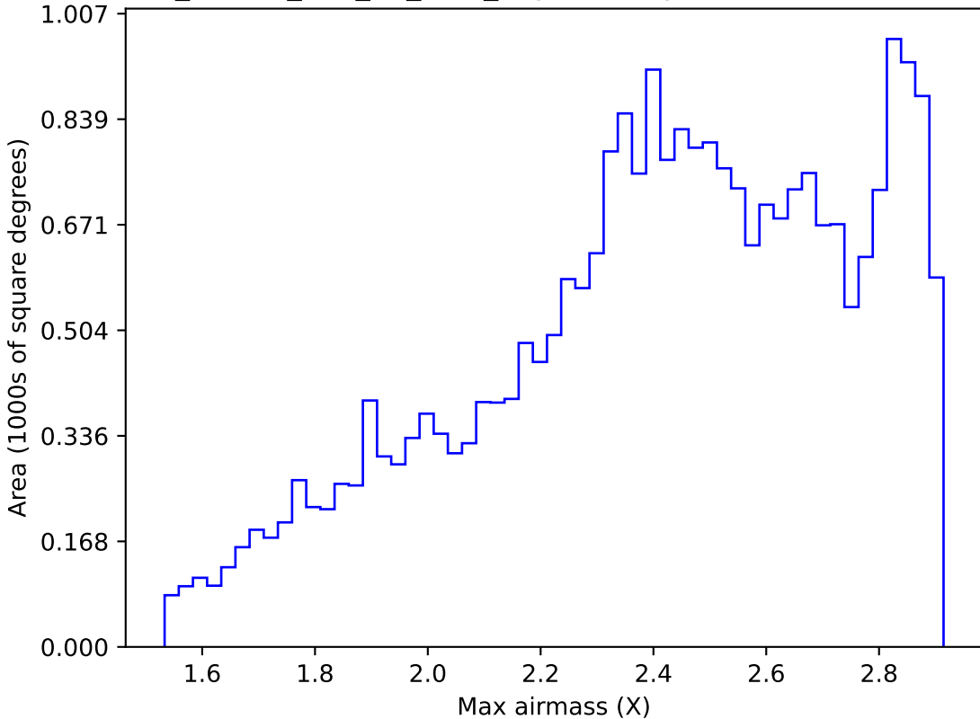
ddf_loaded_half_fl8_v3.4_10yrs All sky i band: Max airmass
