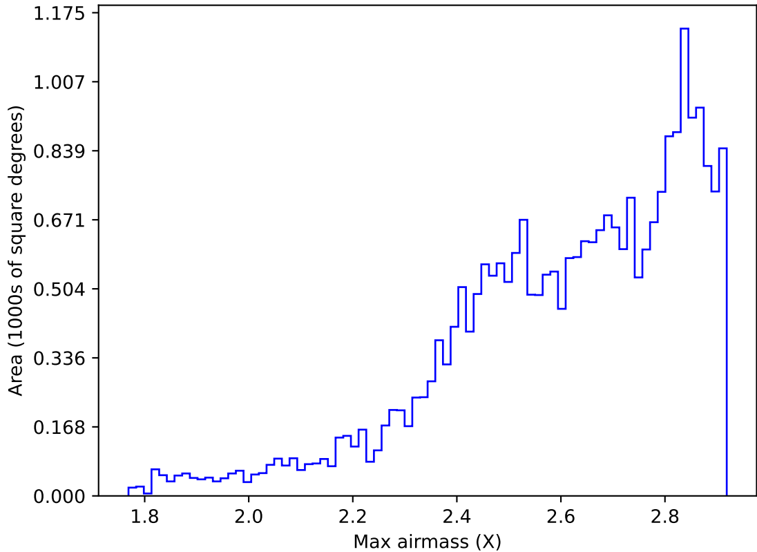
ddf_loaded_half_fl8_v3.4_10yrs All sky all bands: Max airmass
