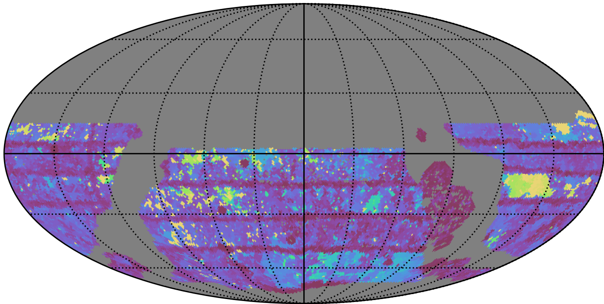
ddf_loaded_half_fl8_v3.4_10yrs WFD z band: Max Inter-Night Gap
