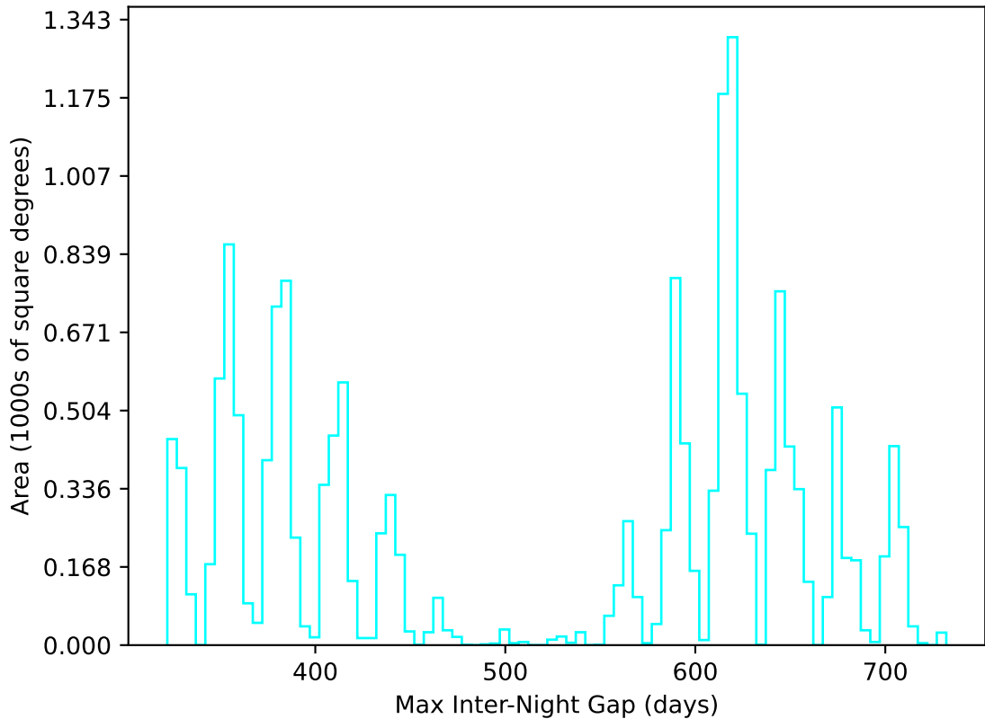
ddf_loaded_half_fl8_v3.4_10yrs WFD u band: Max Inter-Night Gap
