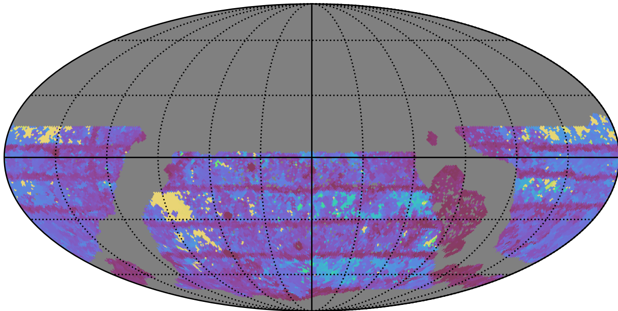
ddf_loaded_half_fl8_v3.4_10yrs WFD r band: Max Inter-Night Gap
