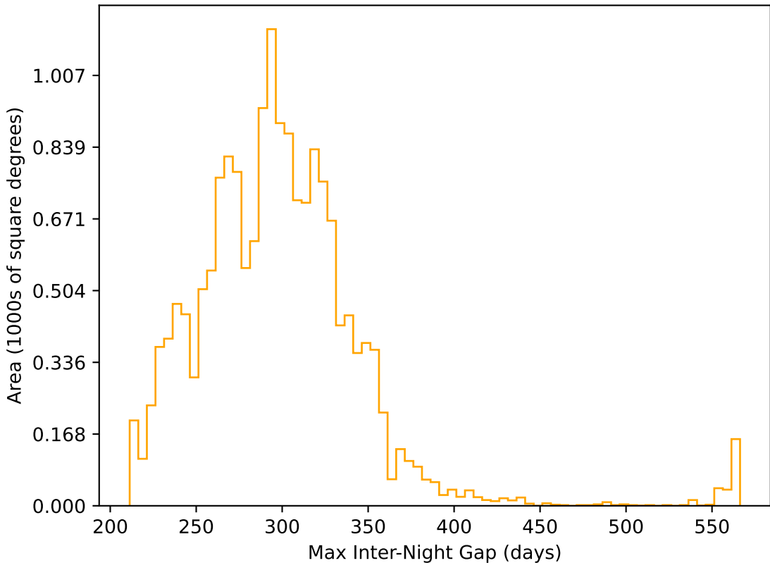
ddf_loaded_half_fl8_v3.4_10yrs WFD r band: Max Inter-Night Gap
