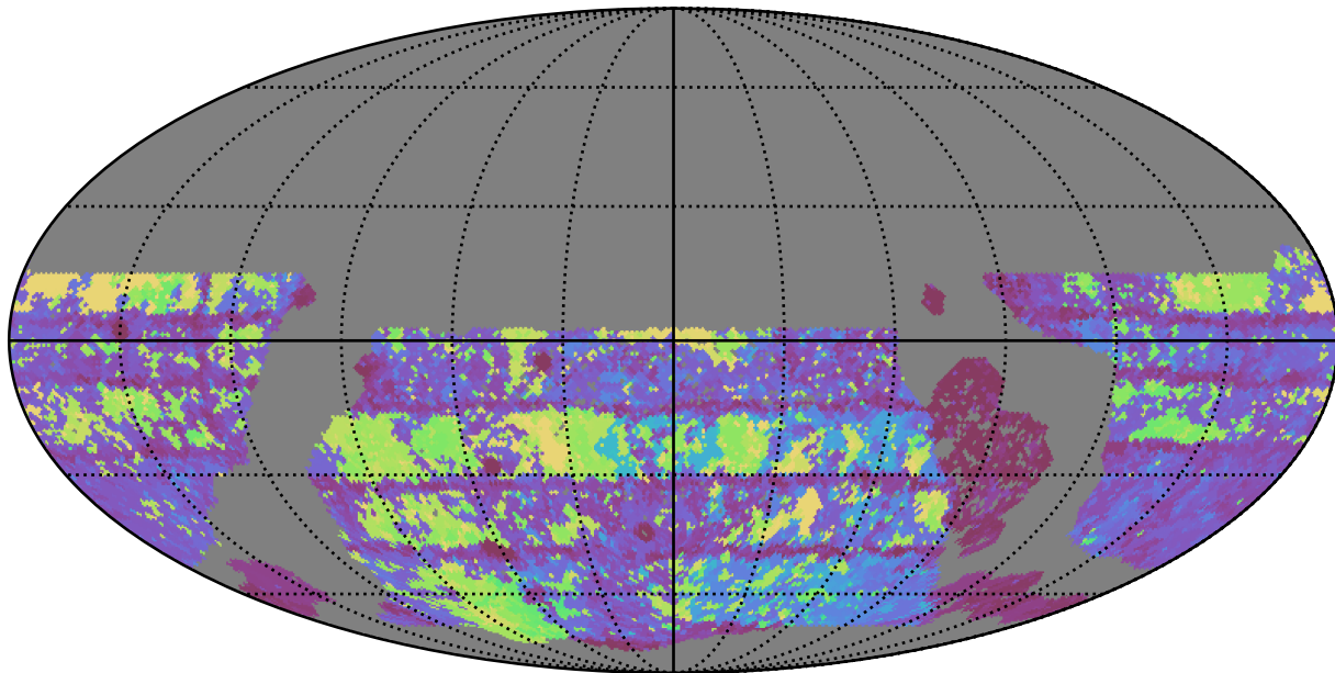
ddf_loaded_half_fl8_v3.4_10yrs WFD g band: Max Inter-Night Gap
