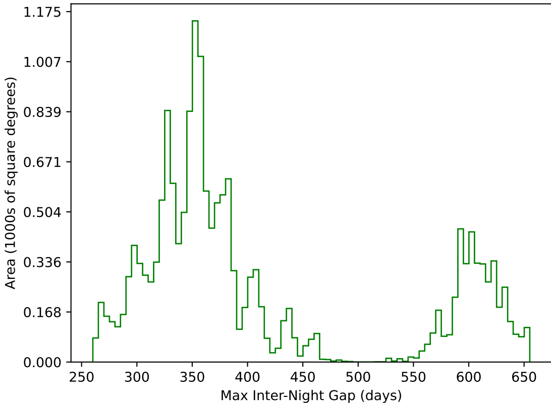
ddf_loaded_half_fl8_v3.4_10yrs WFD g band: Max Inter-Night Gap
