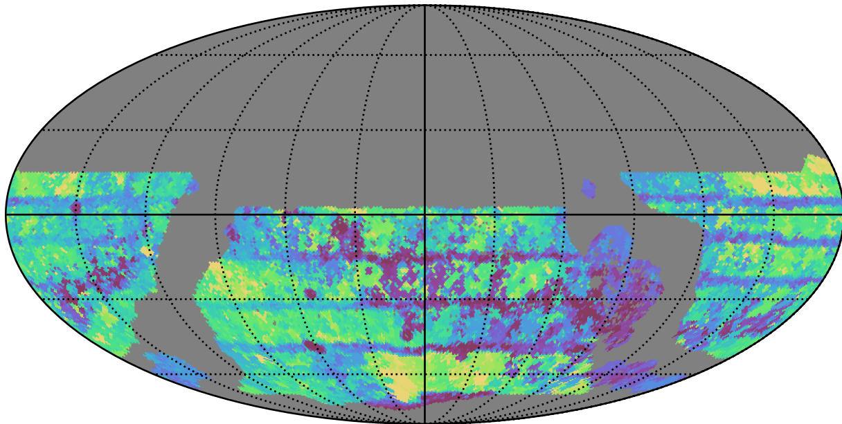
ddf_loaded_half_fl8_v3.4_10yrs WFD all bands: Max Inter-Night Gap
