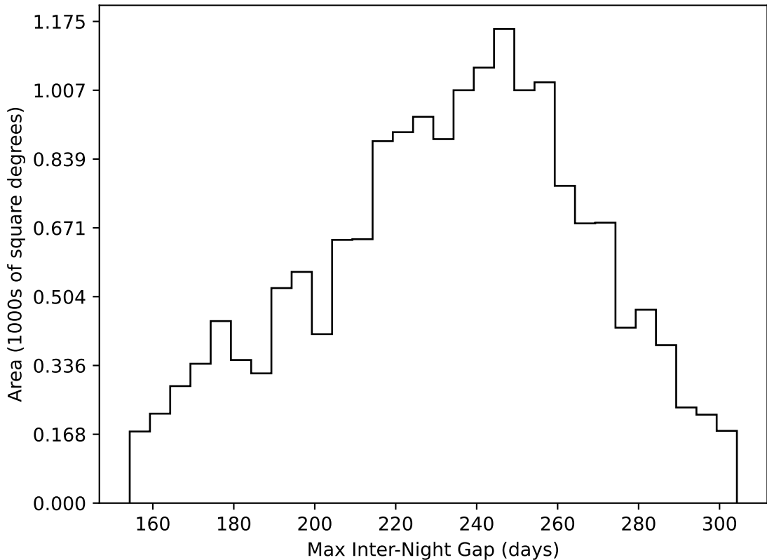
ddf_loaded_half_fl8_v3.4_10yrs WFD all bands: Max Inter-Night Gap
