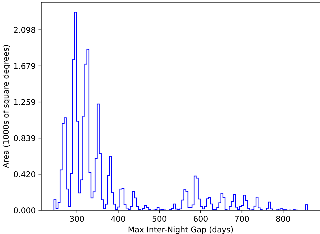
ddf_loaded_half_fl8_v3.4_10yrs All sky y band: Max Inter-Night Gap
