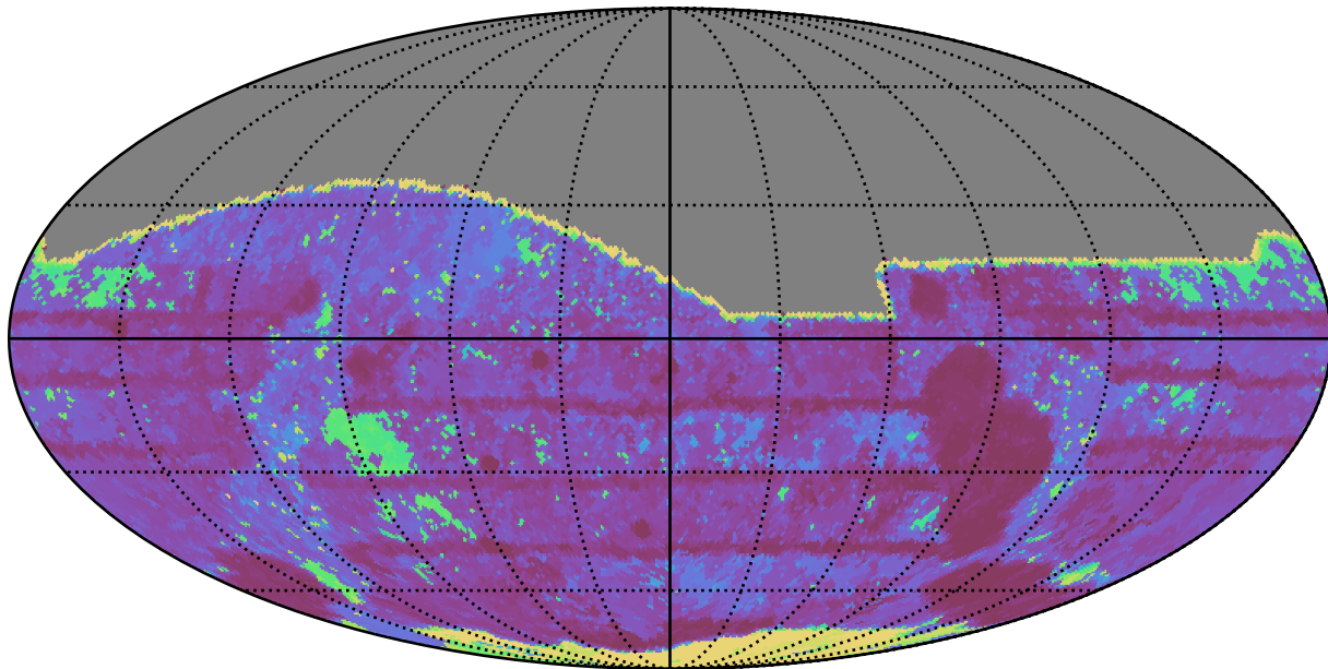
ddf_loaded_half_fl8_v3.4_10yrs All sky r band: Max Inter-Night Gap
