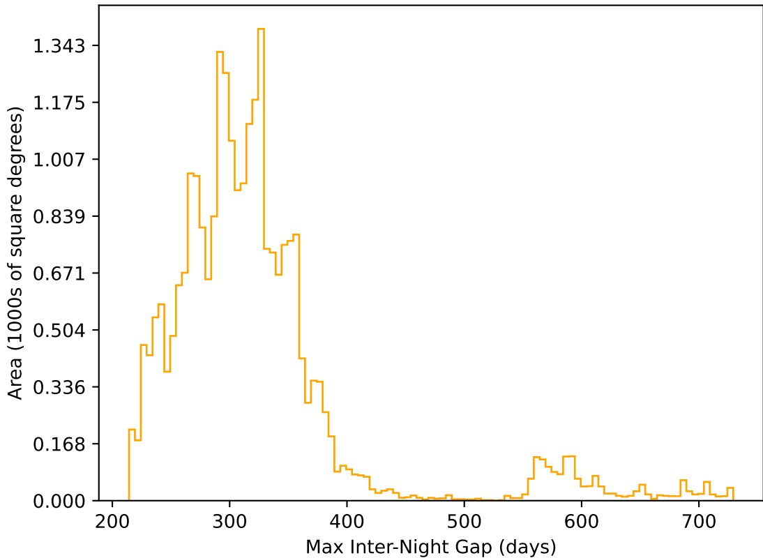
ddf_loaded_half_fl8_v3.4_10yrs All sky r band: Max Inter-Night Gap
