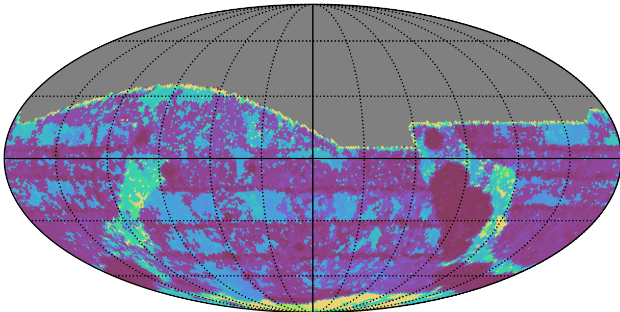
ddf_loaded_half_fl8_v3.4_10yrs All sky g band: Max Inter-Night Gap
