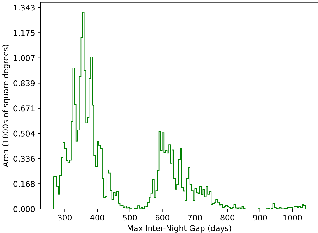
ddf_loaded_half_fl8_v3.4_10yrs All sky g band: Max Inter-Night Gap
