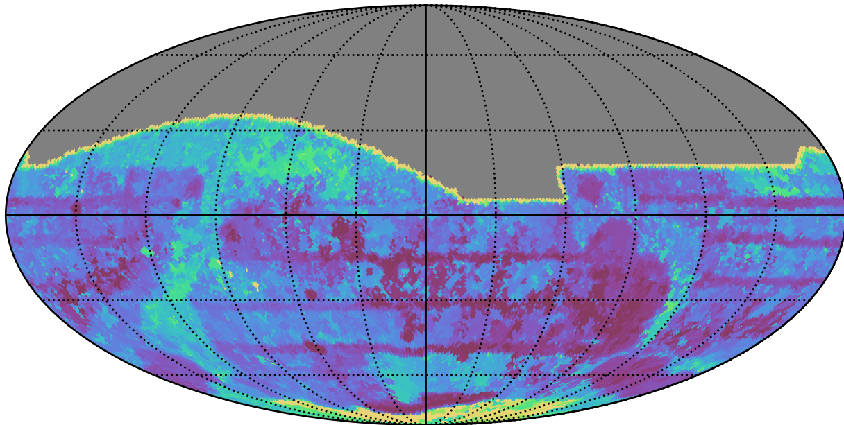
ddf_loaded_half_fl8_v3.4_10yrs All sky all bands: Max Inter-Night Gap
