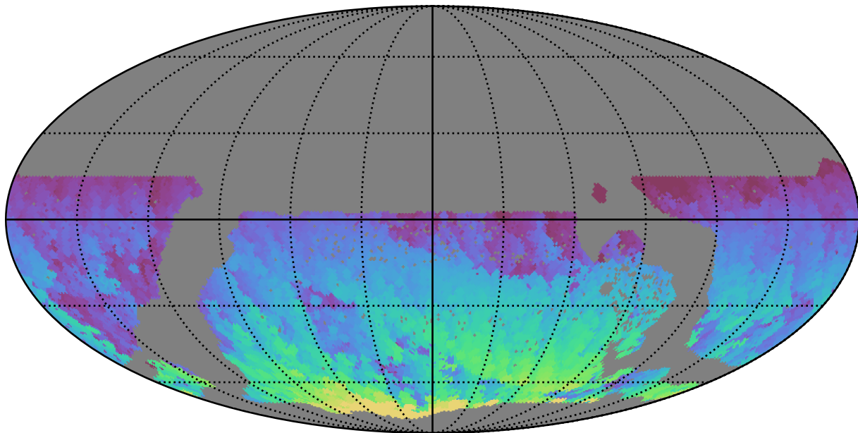
ddf_loaded_half_fl8_v3.4_10yrs WFD z band: Max HA
