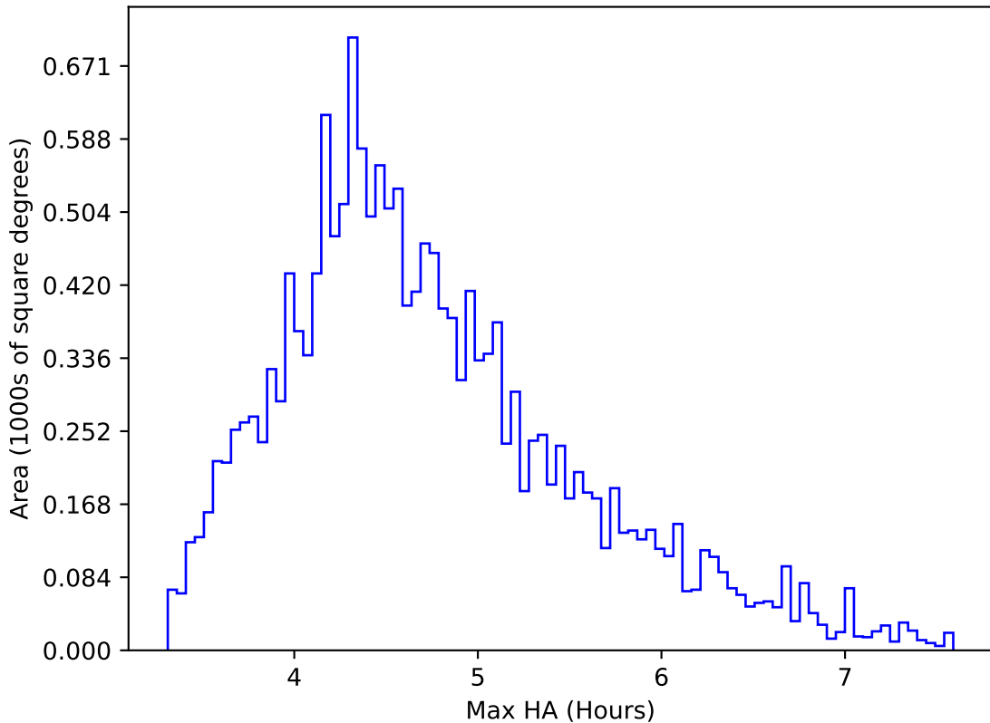
ddf_loaded_half_fl8_v3.4_10yrs WFD y band: Max HA
