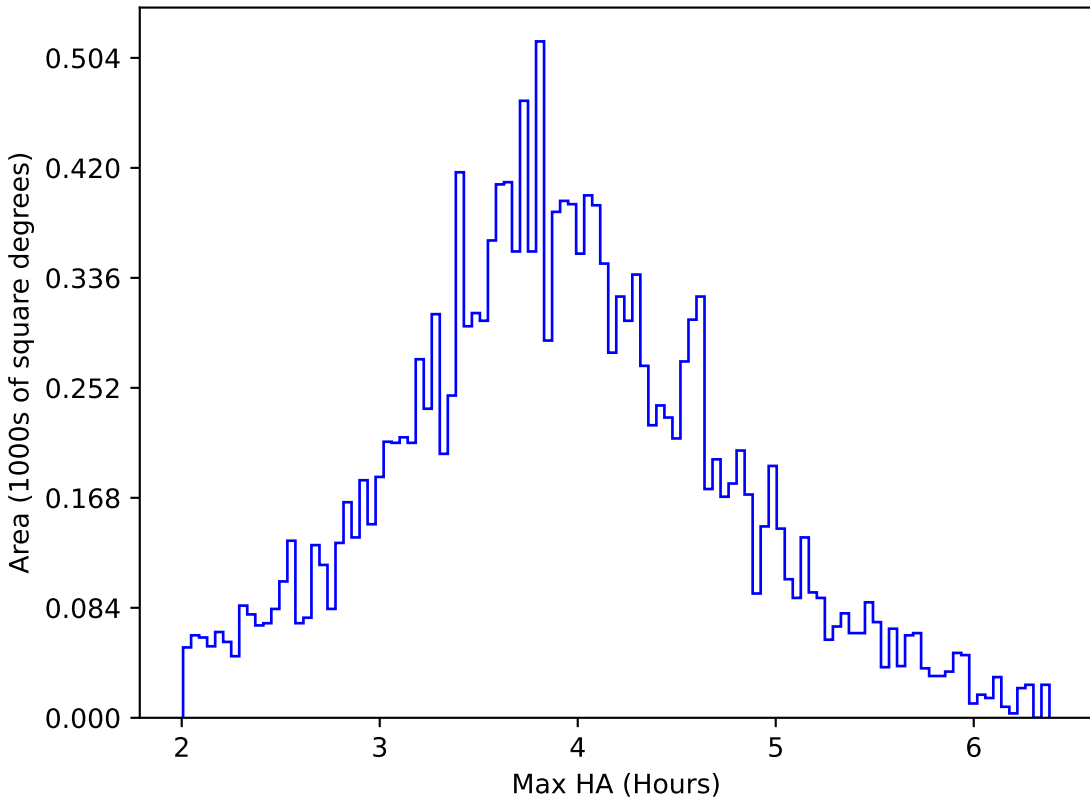
ddf_loaded_half_fl8_v3.4_10yrs WFD u band: Max HA
