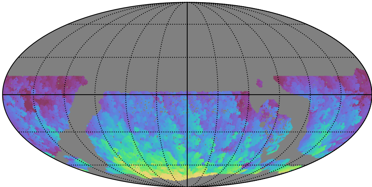
ddf_loaded_half_fl8_v3.4_10yrs WFD r band: Max HA
