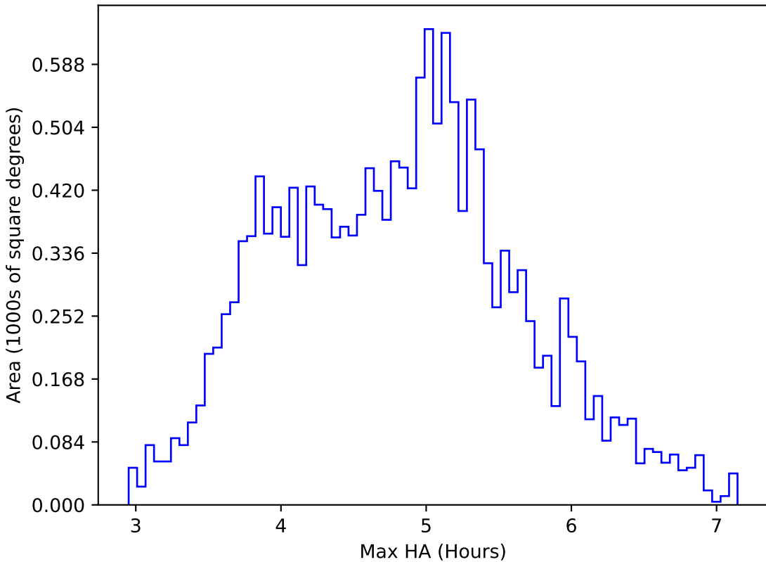
ddf_loaded_half_fl8_v3.4_10yrs WFD i band: Max HA
