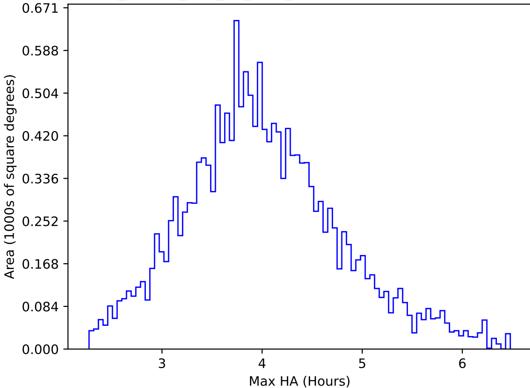
ddf_loaded_half_fl8_v3.4_10yrs WFD g band: Max HA
