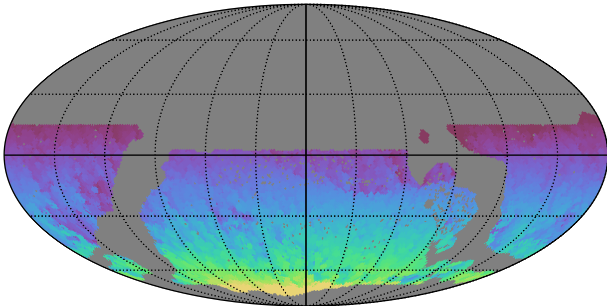
ddf_loaded_half_fl8_v3.4_10yrs WFD all bands: Max HA
