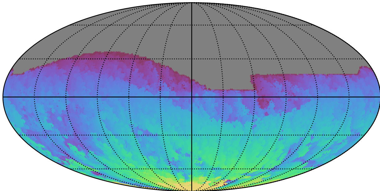
ddf_loaded_half_fl8_v3.4_10yrs All sky z band: Max HA
