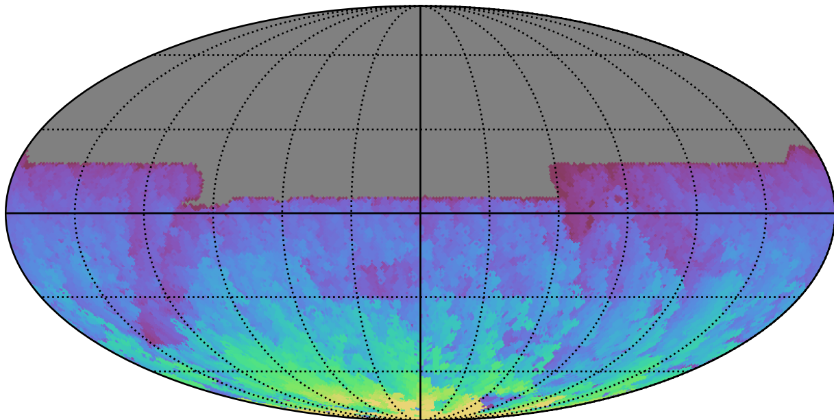
ddf_loaded_half_fl8_v3.4_10yrs All sky y band: Max HA
