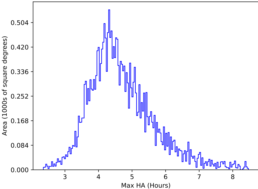
ddf_loaded_half_fl8_v3.4_10yrs All sky y band: Max HA
