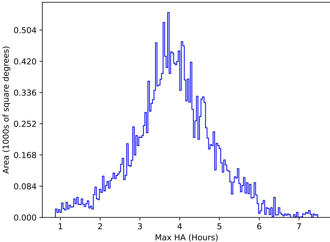
ddf_loaded_half_fl8_v3.4_10yrs All sky u band: Max HA
