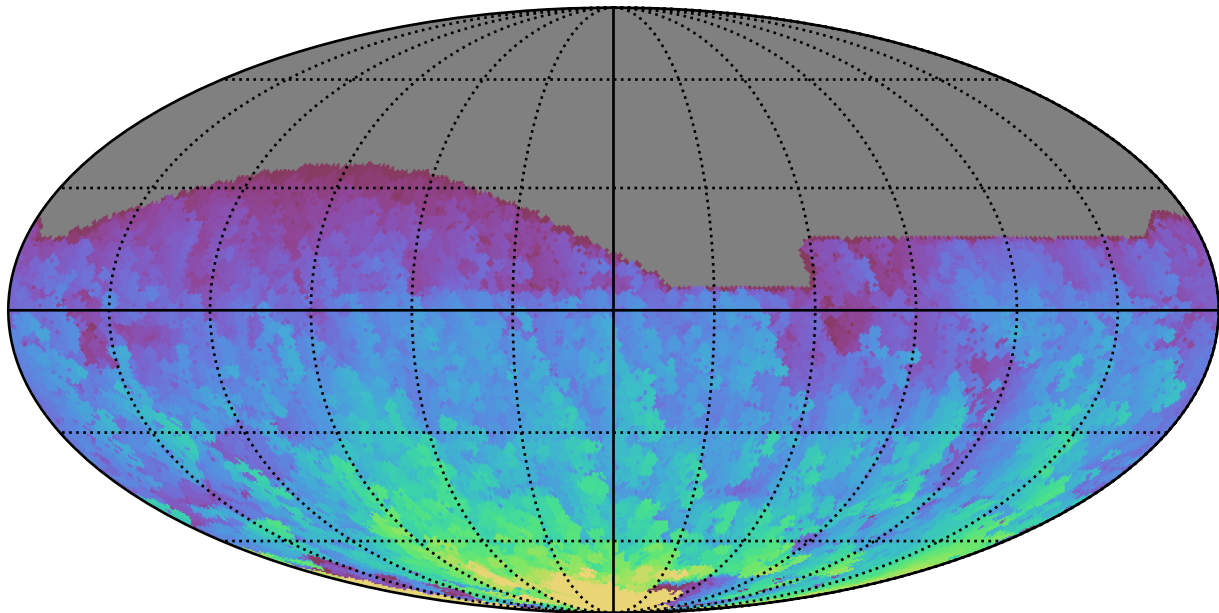
ddf_loaded_half_f18_v3.4_10yrs All sky r band: Max HA
