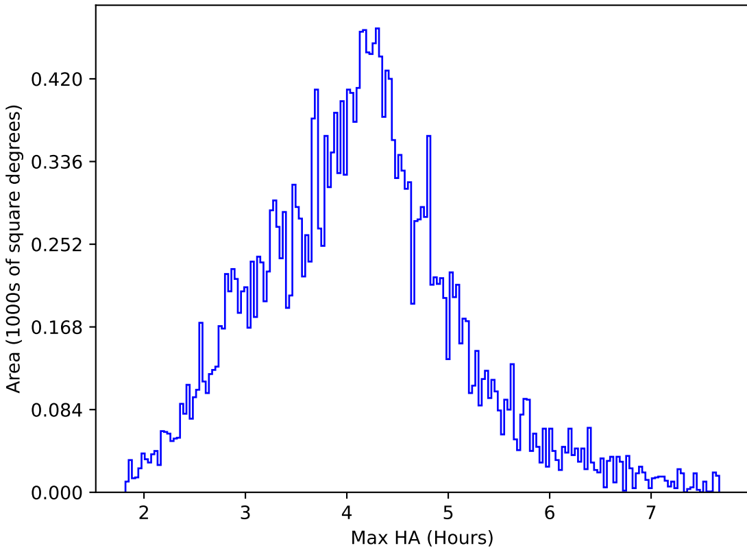
ddf_loaded_half_fl8_v3.4_10yrs All sky r band: Max HA
