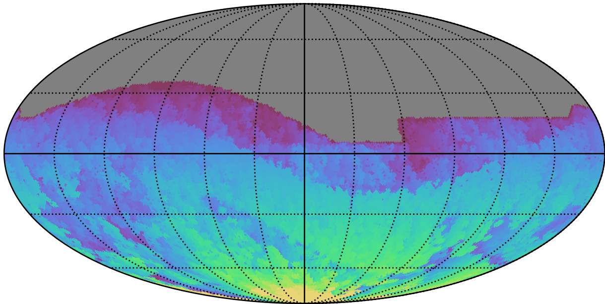
ddf_loaded_half_fl8_v3.4_10yrs All sky i band: Max HA
