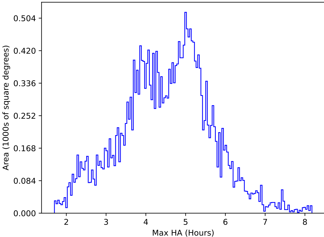
ddf_loaded_half_f18_v3.4_10yrs All sky i band: Max HA
