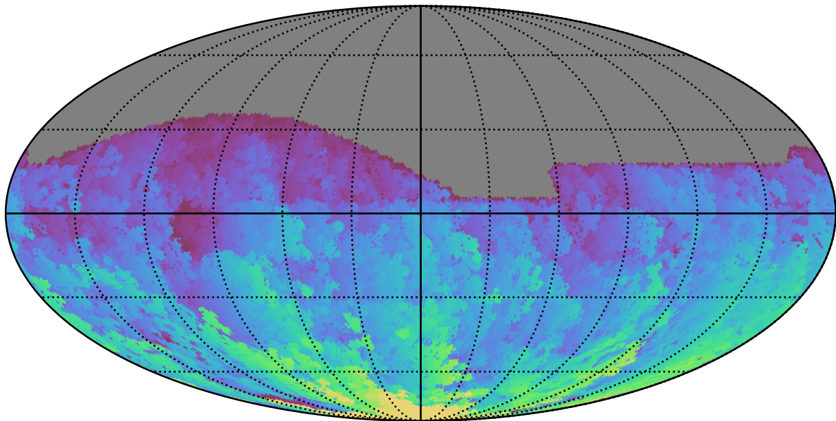
ddf_loaded_half_fl8_v3.4_10yrs All sky g band: Max HA
