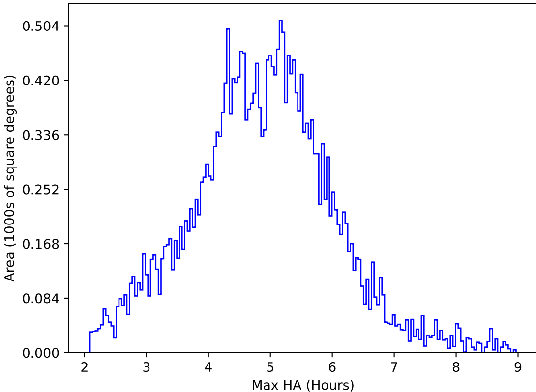
ddf_loaded_half_fl8_v3.4_10yrs All sky all bands: Max HA
