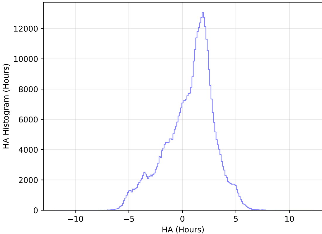
ddf_loaded_half_fl8_v3.4_10yrs WFD z band: HA Histogram
