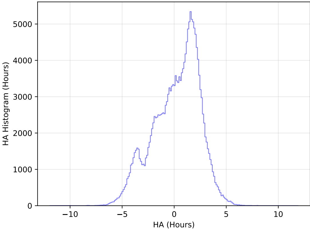
ddf_loaded_half_fl8_v3.4_10yrs WFD g band: HA Histogram
