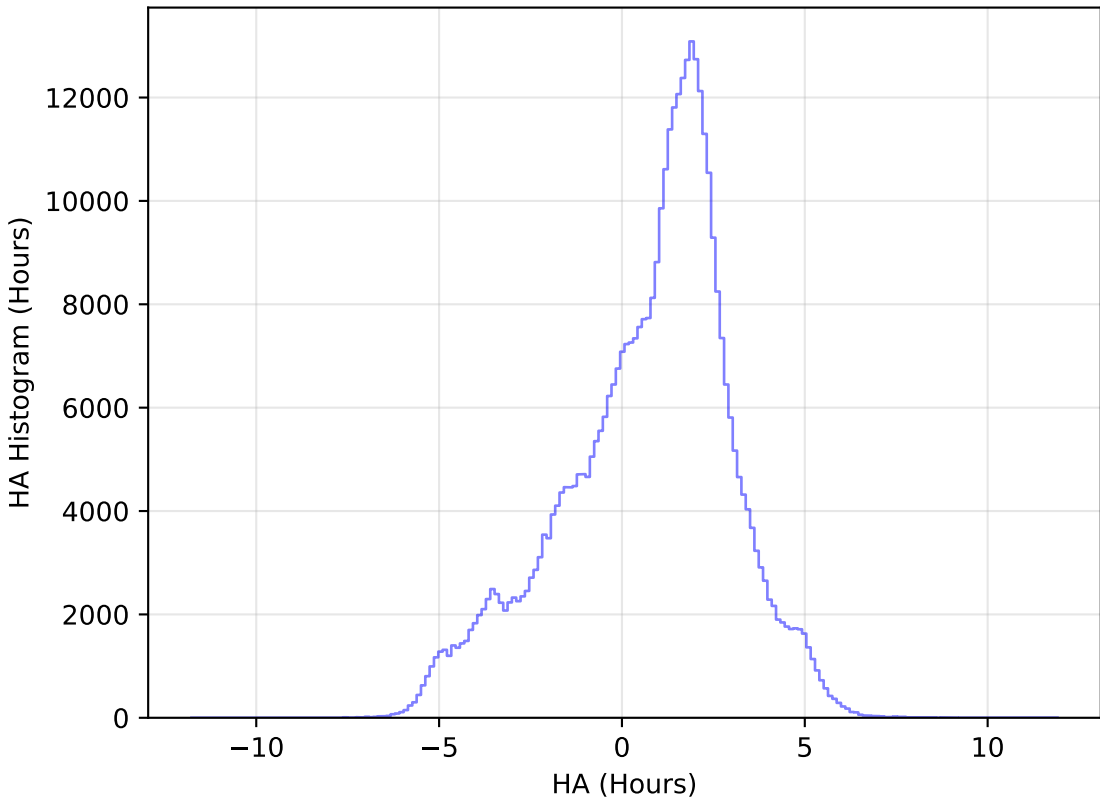
ddf_loaded_half_fl8_v3.4_10yrs All sky z band: HA Histogram
