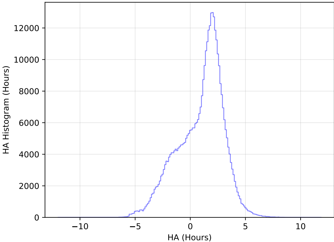
ddf_loaded_half_fl8_v3.4_10yrs All sky y band: HA Histogram
